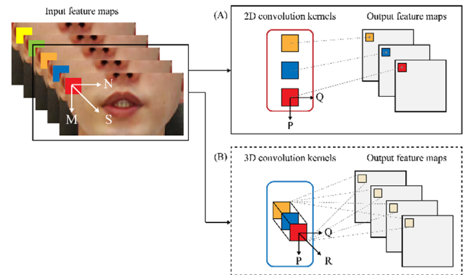
FIGURE 4 Comparison of convolutions in (A) 2D and (B) 3D. The width, length, sequence, height, weight, and 3D kernel of the kernel are denoted by N, M, S, P, Q, and R, respectively.
