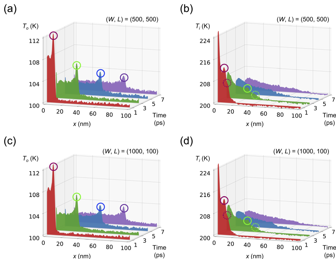
Fig. 6 The decomposed temperature profiles in GNRs along the length at different propagating times: (a) out-of-plane and (b) in-plane temperature for (W, L) = (500, 500) nm, and (c) out-of-plane and (d) in-plane temperature for (W, L) = (1000, 100) nm, respectively. Simulations are conducted at T_{\text{ref}} = 300 K.
