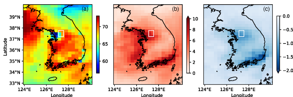
Figure 5. (a) Maximum daily 8 h average (MDA8) ozone (ppb) from 1 May to 10 June 2016, the impact from (b) scaled VOCs as described in Sect. 2, and (c) adding peroxybenzoyl nitrate (PN) chemistry to the simulation in panel (b) described in Sect. 5. The white box designates the Seoul Metropolitan Area (SMA).
