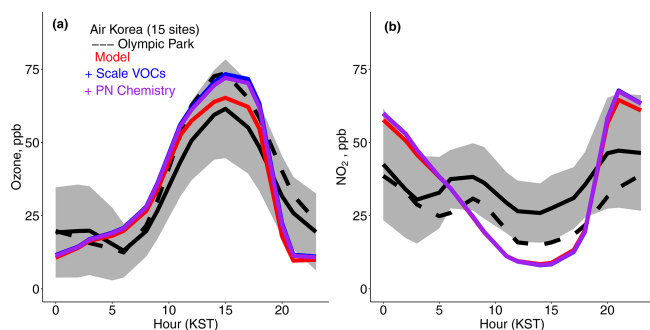
Figure 4. Mean diurnal cycle for (a) ozone and (b) NO 2 for the AirKorea sites within the GEOS-Chem grid box at Olympic Park. The dashed line represents the EPA monitor at Olympic Park (Table 1). The gray shading represents the standard deviation across the AirKorea sites (see Fig. 1b, Travis et al., 2022). KST is Korean standard time (UTC+9).
