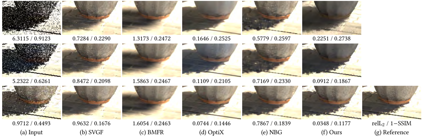
Fig. 5. Comparisons of denoising techniques for the unbiased input (a), generated using three different sampling methods: ordinary path tracing (top row), path tracing with ReSTIR DI (second row), and ReSTIR PT (bottom row). We show the insets from the 100th frame in the image sequence for the BISTRO scene.
