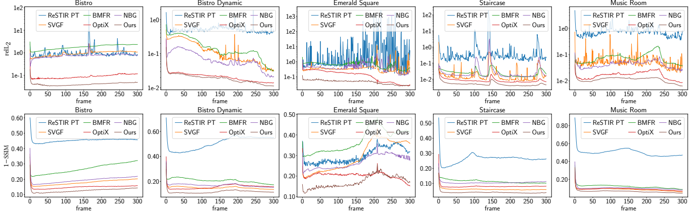
Fig. 7. Relative L_2 ( relL_2 ) and 1-SSIM comparisons of denoising methods for the five scenes, each containing 300 animated frames.
