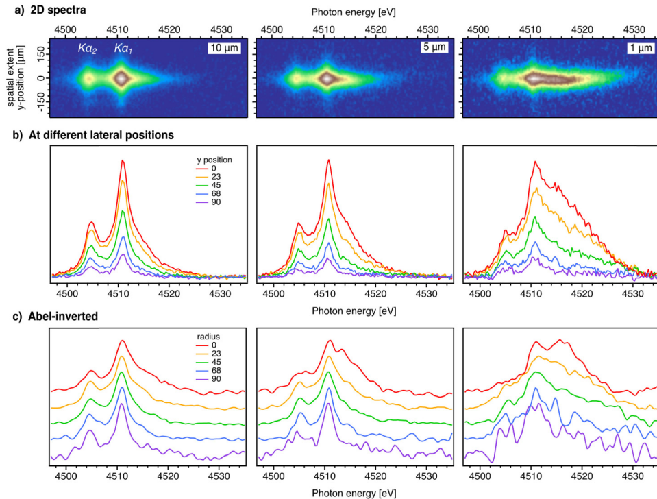
Fig. 2. (a) Averaged K\alpha emission image (top), (b) spectra from different lateral target positions (middle), and (c) Abel-inverted experimental spectra of the warm dense titanium foils of 10, 5, and 1 \mu\text{m} thicknesses (bottom). K\alpha_1 emission strengths are normalized to the unity. For clarity, vertical offsets are applied.
