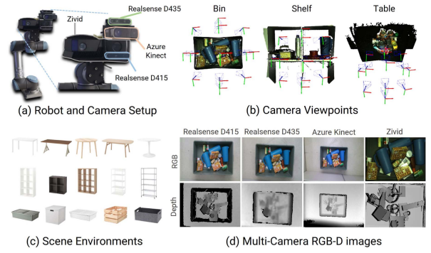
Fig. 3. Multi-camera capture system: (a) a UR5 with four cameras, (b) multiple camera viewpoints, (c) bin, shelf, and table setup, (d) RGB-D image comparison.
