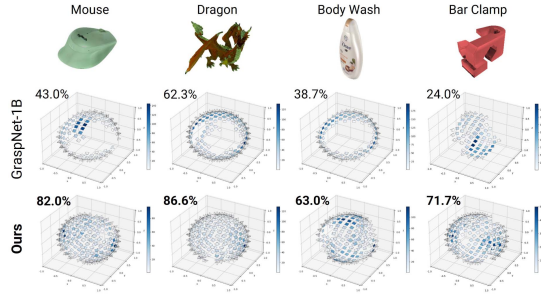
Fig. 6. Viewpoint coverage comparison between GraspNet-1B (top) and GraspClutter6D (bottom). The heatmaps represent object-to-camera orientations discretized into 300 uniform spherical bins. Darker blue indicates high density.
