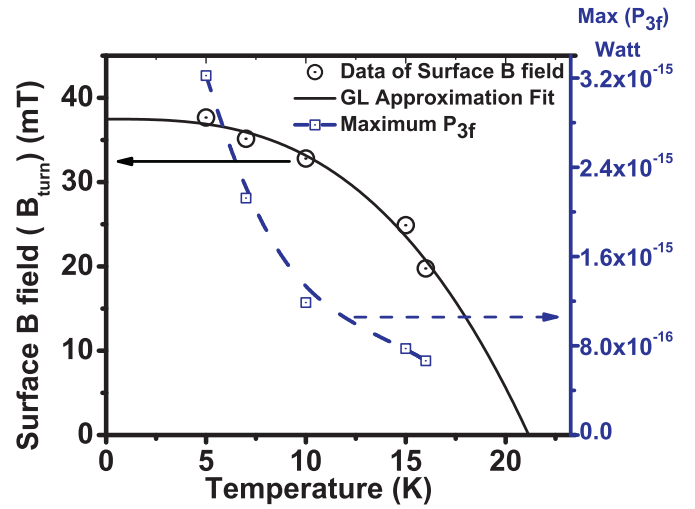
Fig. 6. Temperature dependent estimated surface critical magnetic field ( B_{\text{turn}} ) of \text{Ba}(\text{Fe}_{1-x}\text{Co}_x)_2\text{As}_2 and corresponding P_{3f} (indicated as \text{Max}(P_{3f}) ) in Watts at the turnover point. Note that the dashed line is a B-Spline fit. The solid line is a fit of the surface critical magnetic field from Eq. (1), with T'_c = 21.15 K, n = 2.88 and B_0 = 37.47 mT.
