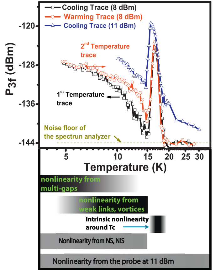
Fig. 3. Temperature dependence of the third harmonic response (log-log plot) for a 200 nm thick \text{Ba}(\text{Fe}_{1-x}\text{Co}_x)_2\text{As}_2 film under 5.1 GHz microwave excitation. The square and circle shapes with inner-centered dot points are experimental P_{3f} data under 8 dBm excitation. The data with blue triangular shape is taken under 11 dBm excitation. The bar plots below the figure indicate different possible nonlinear mechanisms active over different temperature regimes. (For interpretation of the references to colour in this figure legend, the reader is referred to the web version of this article.)
