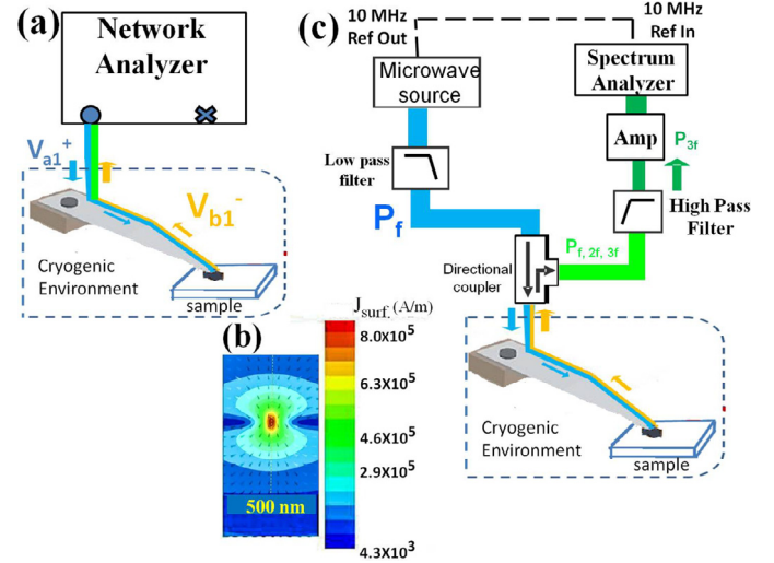
Fig. 1. (a) Schematic diagram of the linear response measurement, S_{11} , performed as a function of temperature with the network analyzer. Note that only one port (marked with a • symbol) is used in the measurement. (b) A simulated surface current density distribution ( J_{\text{surf}} ) on the sample surface created by the magnetic write head probe at the driving frequency is shown, assuming the probe height is 200 nm away from the sample surface [25]. (c) Schematic set up of the third harmonic measurement in nonlinear microwave microscopy. Note that the third harmonic signal ( P_{3f} ) is selectively filtered by the microwave circuit outside the cryogenic environment.
