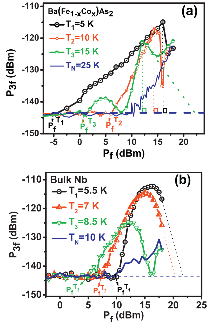
Fig. 5. (a) Dependence of P_{3f} on P_f for a 200 nm thick Ba(Fe 1-x Co x ) 2 As 2 film under 5.1 GHz local microwave excitation. The vertical dashed lines for T_1 = 5 K and T_2 = 10 K indicate the turnover point. Another dashed line on the T_3 = 15 K curve indicates the extrapolation of P_{3f} on P_f through the probe nonlinearity, P_{3f}^{\text{probe}} , which is taken at T_N = 25 K above the T_c of the Ba(Fe 1-x Co x ) 2 As 2 film. The horizontal dashed line indicates the noise floor ( \sim -143 dBm) of the spectrum analyzer. (b) Power dependence of P_{3f} on P_f for a bulk Nb sample under 5.36 GHz local microwave excitation [27]. The dashed line in each curve indicates the extrapolation of P_{3f} on P_f through the P_{3f}^{\text{probe}} to the noise floor of the spectrum analyzer. The T_c of this bulk Nb is 9.2 K and P_{3f}^{\text{probe}} is taken at T_N = 10 K.
