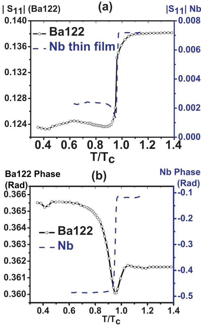
Fig. 2. The temperature dependent linear response S_{11} of the \text{Ba}(\text{Fe}_{1-x}\text{Co}_x)_2\text{As}_2 film measured with the near-field microwave microscope. Both (a) amplitude and (b) of S_{11} phase show a transition at normalized T/T_c = 1 . The same measurement for (a) amplitude and (b) phase of S_{11} is also done on a Nb thin film as shown in blue dash lines for comparison. Note the T_c for the \text{Ba}(\text{Fe}_{1-x}\text{Co}_x)_2\text{As}_2 film and the Nb film are 18.1 K and 8.3 K, respectively. (For interpretation of the references to colour in this figure legend, the reader is referred to the web version of this article.)
