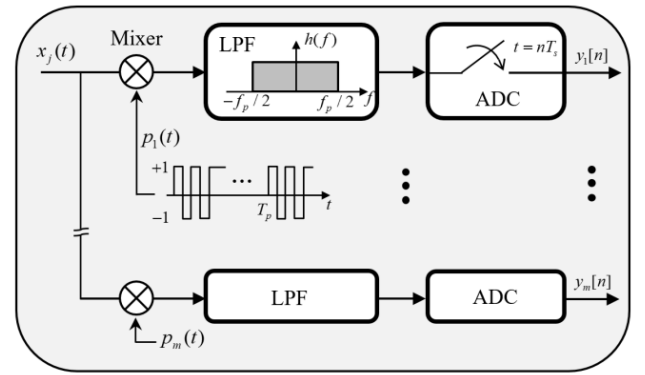
FIGURE 2. Analog module of the MWC.
