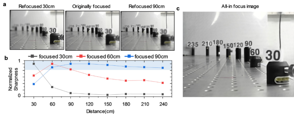
Fig. 6. Results of light-field image processing. (a) Image of light-field refocusing processing. (b) Normalized sharpness graph of the refocused image at 30, 60, and 90 cm. (c) All-in-focus image by using the focal stacking method.
