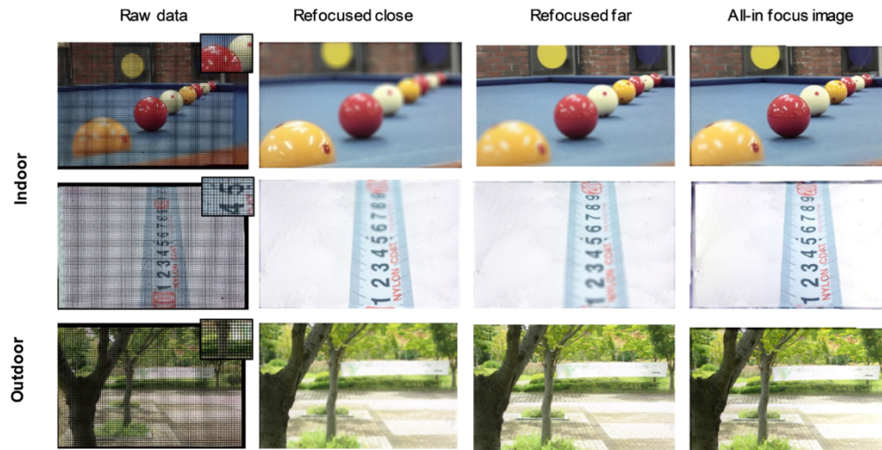
Fig. 7. Test of the light field camera for practical use. Two indoor tests include billiard and tape measure object for general intensity and zoomed-in objects. Outdoor test for a rich light intensity object. Refocusing process was performed for various distances with 3 different conditions. (see Visualization 1 , Visualization 2 , Visualization 3 ).
