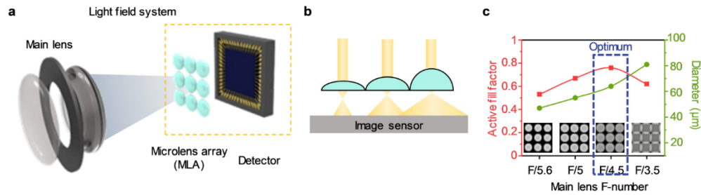
Fig. 1. Description of a light field camera based on microlens array (MLA). (a) Schematic of a light-field camera based on MLA. (b) Difference in the focusing ability of MLA based on the radius of curvature (RoC). (c) Plot of an active fill factor with different F-numbers of the main lens. The F-number of the MLA is 4. This indicates that F-number matching between the main lens and MLA is imperative in terms of minimizing discarded pixels.
