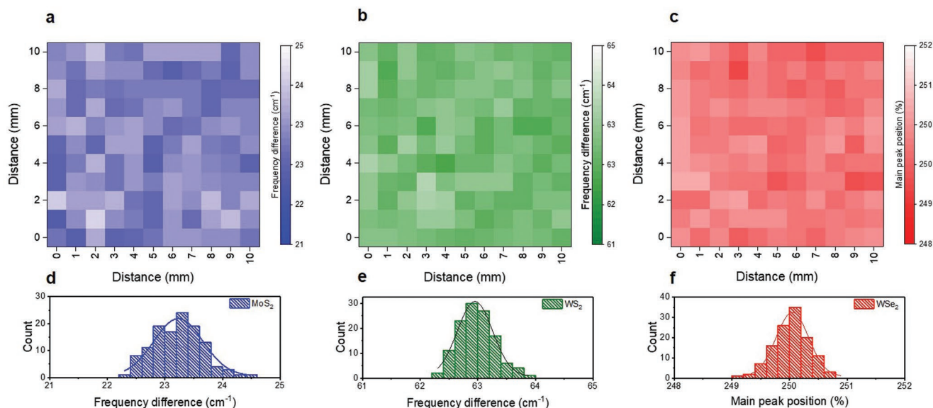
Figure 3. The Raman mapping based on \Delta f values for a) the MoS 2 layer and b) WS 2 layer in the 112-MWW'/p-Si thin film. c) Main peak-position-based Raman mapping for the WSe 2 layer in 112-MWW'/p-Si thin film. Histogram as a function of \Delta f values for d) MoS 2 and e) WS 2 layer calculated from Raman maps in panels (a) and (b). f) Histogram as a function of the main peak position calculated from the Raman map in panel (c).
