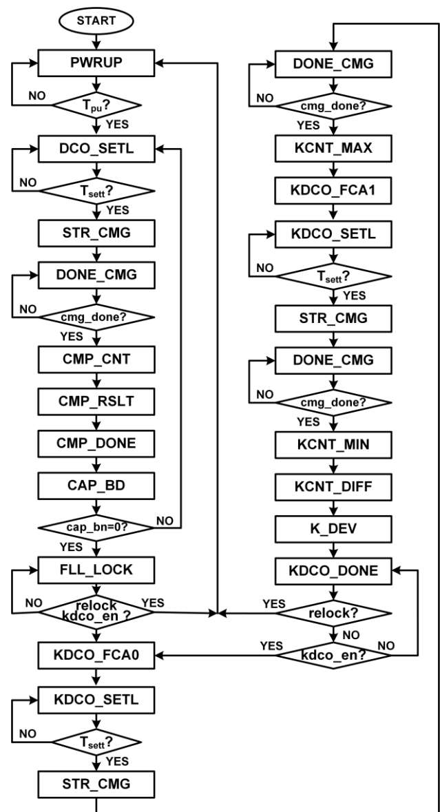
FIGURE 4. FMC finite state machine.
