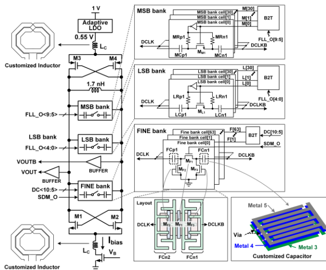
FIGURE 8. DCO design.
