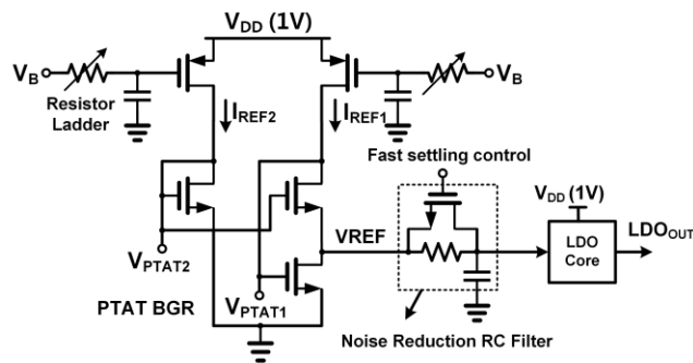
FIGURE 9. Adaptive LDO design.
