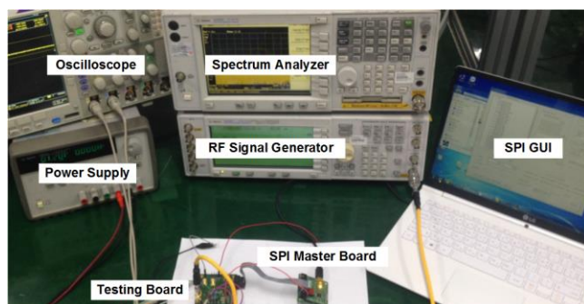
FIGURE 11. Measurement lab setup.
