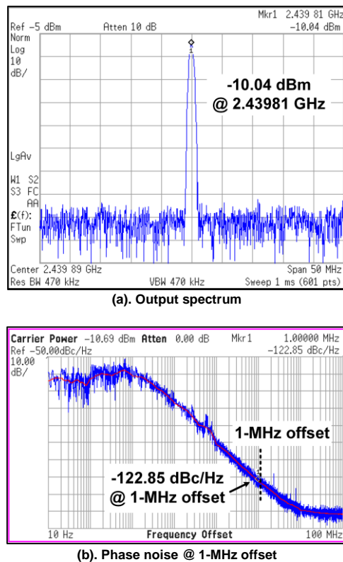
FIGURE 13. DCO output spectrum and phase noise measurement
