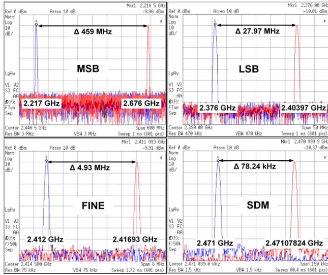
FIGURE 15. Frequency step measurement for MSB, LSB, FINE and SDM.
