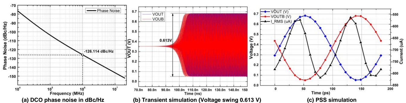
FIGURE 20. DCO simulation analysis.
