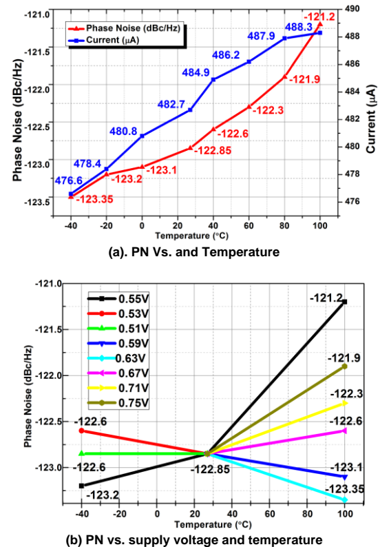
FIGURE 14. DCO measurement results with different conditions.
