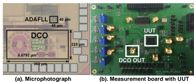
FIGURE 10. Chip microphotograph and measurement board.
