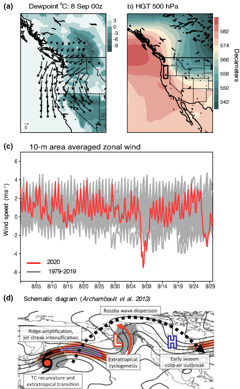
Figure 1. (a) Dewpoint temperature ( ^{\circ}\text{C} ) and 10-m winds at the onset of the wind event that rapidly spread fires in Oregon and Northern California. (b) \text{HGT}_{500} at the same time, showing a stark pressure-gradient centered over the Pacific Northwest. (c). Area averaged 10-m zonal wind speeds for August through September. The black rectangle in panel b indicates the area used for the area average ( 124^{\circ}\text{W} – 121^{\circ}\text{W} and 41^{\circ}\text{N} – 46^{\circ}\text{N} ). (d) Schematic diagram illustrating the process in which a recurving typhoon impacts the downstream flow (Archambault et al., 2013).
