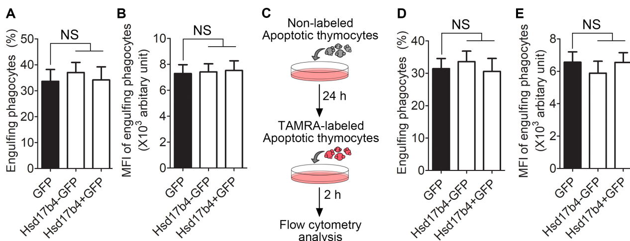
Fig. 5. Hsd17b4 is unlikely to be involved in efferocytosis. (A and B) LR73 cells transfected with the indicated plasmids were incubated with TAMRA-labeled apoptotic thymocytes for 2 h, extensively washed with ice-cold PBS, trypsinized, and analyzed by flow cytometry. Cells double-positive for GFP and TAMRA were considered to be phagocytes engulfing apoptotic cells. NS, not significant. (C) Schematic diagram of the assay used to assess continuous efferocytosis. (D and E) LR73 cells transfected with the indicated plasmids were incubated with the same number of unstained apoptotic cells. After incubation for 24 h, LR73 cells were incubated with TAMRA-stained apoptotic cells for 2 h, and then LR73 cells engulfing TAMRA-stained apoptotic cells were analyzed by flow cytometry.
