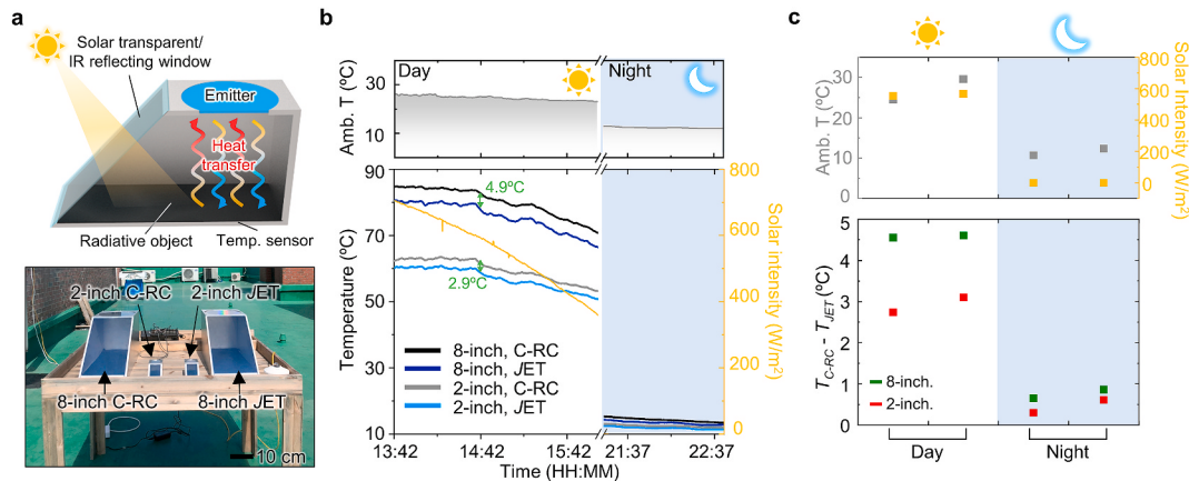
Fig. 5. (a) Schematic illustration (top) and photograph of measurement setup, designed in the shape of an automobile. (b) Temperature measurement of radiative object for different emitters (i.e., C-RC and JET) with 8-inch and 2-inch size. (c) Measurements for two days and nights with different weather conditions of solar intensity and ambient temperature.
