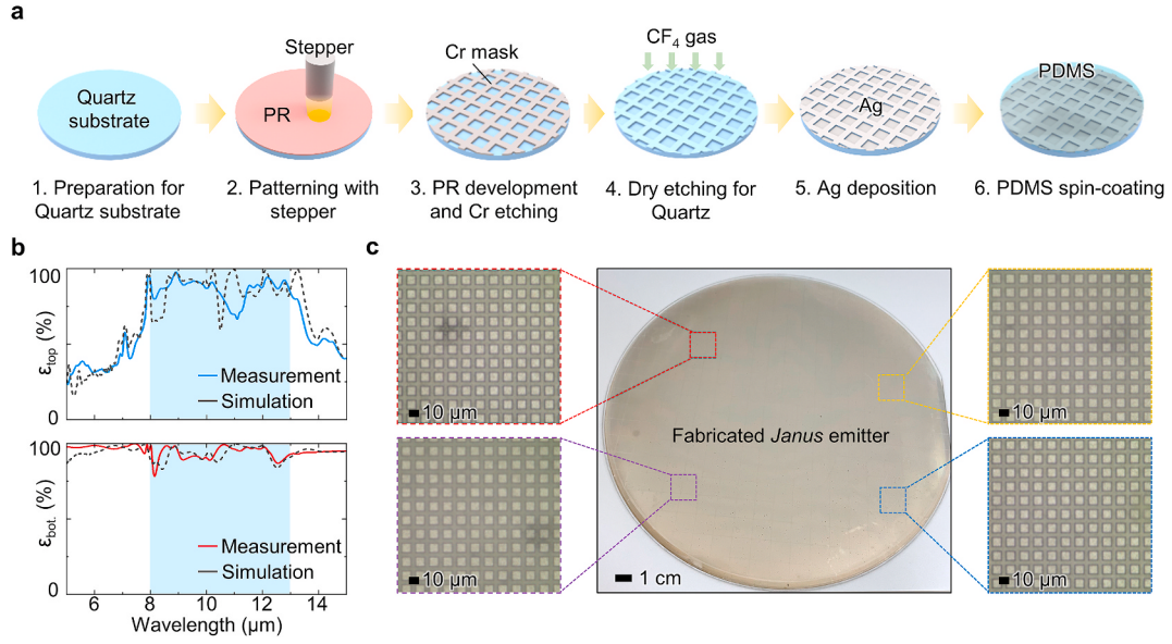
Fig. 2. (a) Fabrication process of JET using MEMS methods for large-area emitter. (b) Measured and simulated emissivity spectra of designed JET at the top side ( \epsilon_{top} ) and the bottom side ( \epsilon_{bot} ) which shows selective and broadband emissions respectively. (c) The optical image of fabricated 8-inch sized JET (middle) with microscopic images at different regions in Janus emitter.
