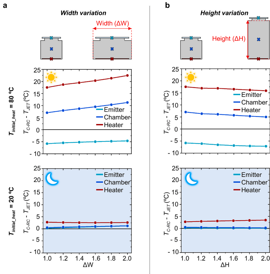
Fig. 4. The calculated temperature difference between the cases using C-RC and JET at the center of emitter, chamber, and heater as a function of (a) width and (b) height. The initial value is set to 80^\circ\text{C} (top) and 20^\circ\text{C} (bottom).
