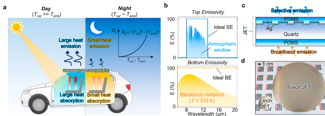
Fig. 1. (a) Schematic of Janus emitter (JET) on an enclosed automobile, where heat is trapped by the greenhouse effect. JET allows large heat emission from space in the daytime while small heat emission in the nighttime. (b) Emissivity spectra of Ideal JET which shows selective emission at the top side, and broadband emission at the bottom side. (c) Cross-sectional schematic of our designed JET, composed of PDMS layers, Ag layer, and micro-patterned quartz. (d) The optical image of fabricated 2-inch and 8-inch sized JET.
