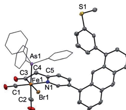
Fig. 1 ORTEP representation (30% thermal ellipsoids) for [(\text{Anth} \cdot \text{C}^{\text{H}_2}\text{NS}^{\text{off}})\text{Fe}(\text{CO})_2(\text{Br})(\text{AsPh}_3)] . Hydrogen atoms are omitted for clarity and the phenyl groups of AsPh 3 are depicted as wireframes. Selected bond distances (Å) and bond angles (°): Fe1–C3 = 1.942(3), Fe1–N1 = 2.036(2), Fe1–As1 = 2.4050(5), C3–Fe1–N1 = 83.55(11), C3–Fe1–As1 = 91.76(11), N1–Fe1–As1 = 88.97(6).
