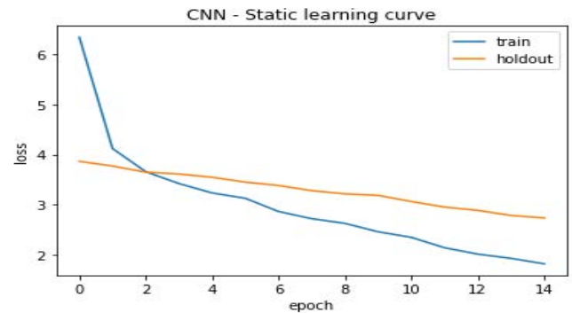
FIGURE 4. Training and hold-out set performance trend over epoch in terms of the loss in case of CNN-static.
