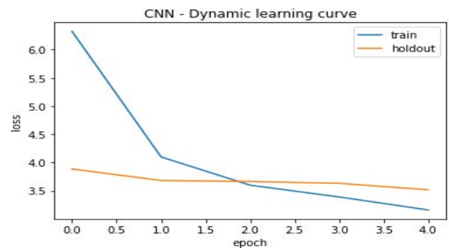
FIGURE 5. Training and hold-out set performance trend over epoch in terms of the loss in case of CNN-dynamic.
