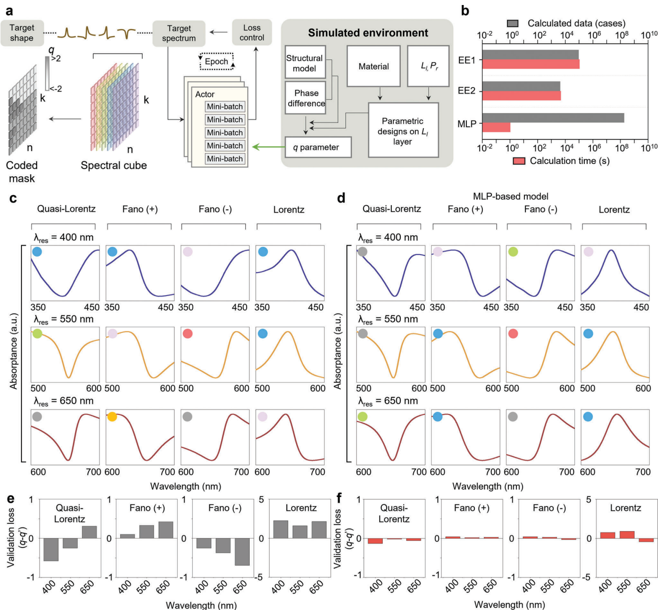
Figure 4. Spectral shape calculation and performance evaluation of MLP model. a) Computational modeling of Fano resonator composed of Resonators 1 and 2 and flow chart of MLP algorithm. b) Comparison of computation times for EE1 (resonator 1: six materials, thickness gap of 1 nm, porosity gap of 1%, resonator 2: thickness gap of 1 nm), EE2 (resonator 1: six materials, thickness gap of 5 nm, porosity gap of 5%, resonator 2: thickness gap of 5 nm) and MLP. Computation times for EE1, EE2, and MLP. c,d) Reflectance spectra obtained using c) EE2 and d) MLP model. Each circle is color-coded to indicate the type of lossy material. e,f) Validation loss ( q-q' ) of the spectra obtained using e) EE2 and f) MLP model.
